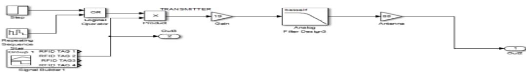
Figure 1.6: Simulink model of an RFID transmitter
