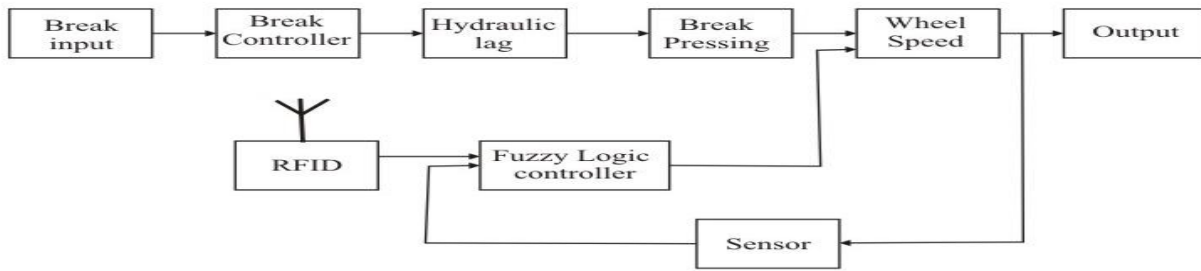
Fig 1.2: Block diagram of a vehicle speed controller with RFID and Fuzzy controller.
